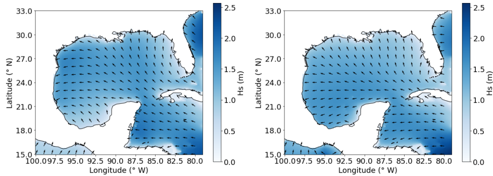
FIGURE 3.3: Left: H_s Significant wave height (colours) and wave direction (arrows) averaged between 12Z 06/03/2022 and 12Z 12/03/2022. Right: The same averaged between 12Z 13/03/2022 and 12Z 19/03/2022
