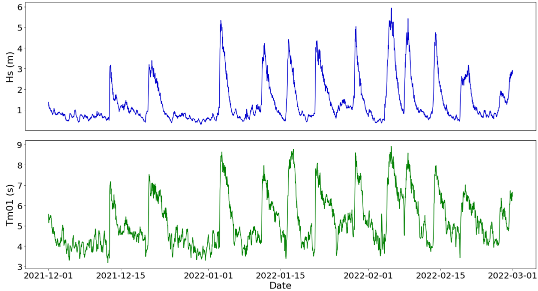
FIGURE 3.8: Times series of observed Hs (top) and Tm01 (bottom) over a three-month period from 01/12/2021 to 01/03/2022
