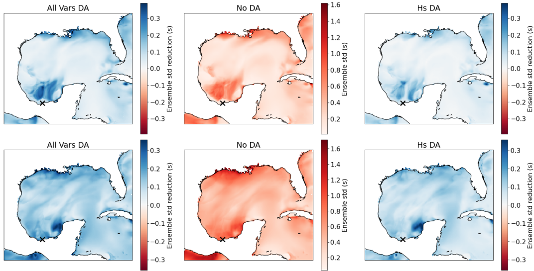
FIGURE 5.9: Ensemble standard deviation in Tm01 at 12Z 11/03/2022, taken from 12Z 06/03/2022 (top) and 12Z 10/03/2022 (bottom) model runs. Middle panel shows standard deviation from no DA, side panels show standard deviation reduction from all vars DA (left) and Hs DA (right).
