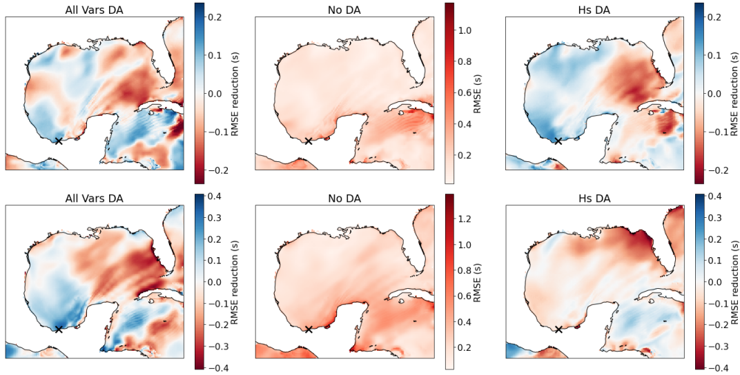
FIGURE 4.5: Maps of RMSE in Tm01 ensemble mean from the period 12Z 12/03/2022 to 13/03/2022, with leadtime 2-3 days (top) and 4-5 days (bottom). Middle panels show RMSE from no DA, side panels show absolute RMSE reduction compared to no DA from all vars DA (left) and Hs DA (right). The buoy location is marked with a cross.
