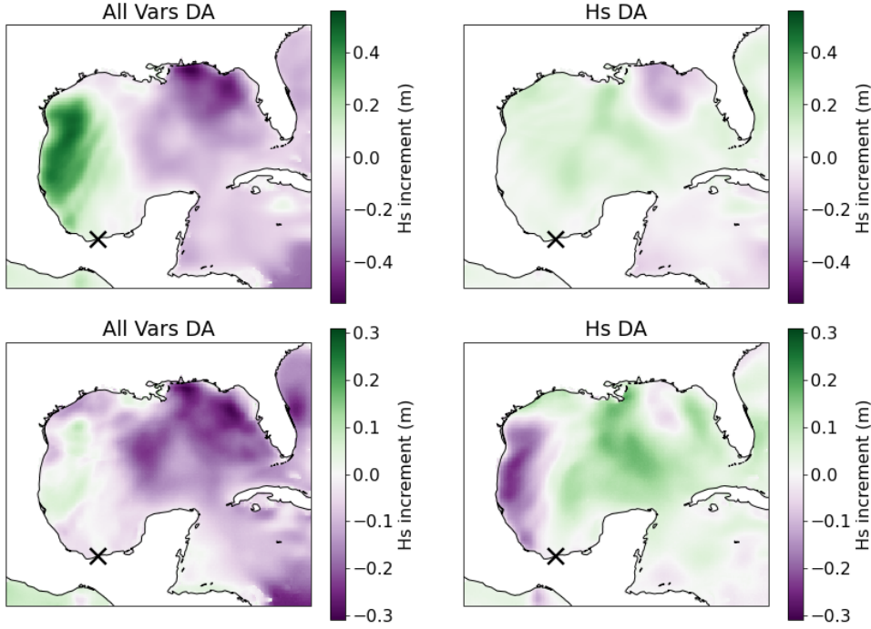
FIGURE 4.10: Hs increments at 12Z 15/03/2022 from all vars DA (left) and Hs DA (right). Taken from 12Z 10/03/2022 forecast run ensemble member 10 (top) and ensemble mean (bottom). The buoy location is marked with a cross.
