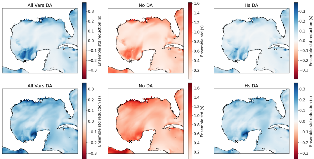
FIGURE 4.8: Ensemble standard deviation in Tm01 at 12Z 11/03/2022, taken from 12Z 06/03/2022 (top) and 12Z 10/03/2022 (bottom) model runs. Middle panel shows standard deviation from no DA, side panels show standard deviation from all vars DA (left) and Hs DA (right).
