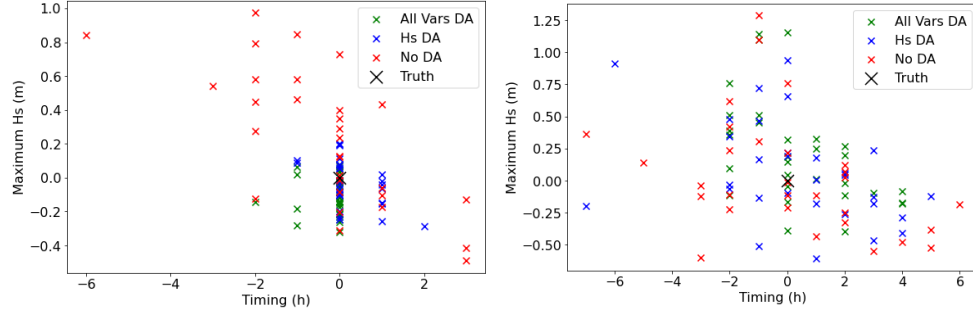
FIGURE 4.9: Scatter plots of timing and magnitude of maximum Hs at buoy location from period 12Z 12/03/2022 to 12Z 13/03/2022. Generated from model run starting 12Z 10/03/2022 (left) and 12Z 08/03/2022 (right). Truth is shown in black, and the no DA, Hs DA and all vars DA ensemble members are shown in red, blue and green respectively.
