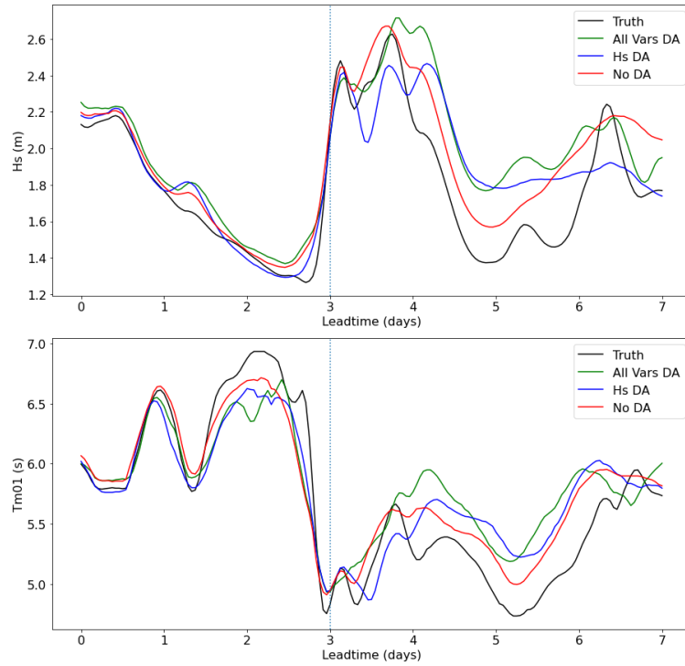
FIGURE 4.2: Timeseries of Hs (top) and Tm01 (bottom) at 30°N 80° W from 12Z 09/03/2022 model run. No DA ensemble mean is shown in red, Hs DA ensemble is shown in blue, all vars DA ensemble mean is shown in green and truth is shown in black. Blue dotted line indicates the end of the assimilation window.
