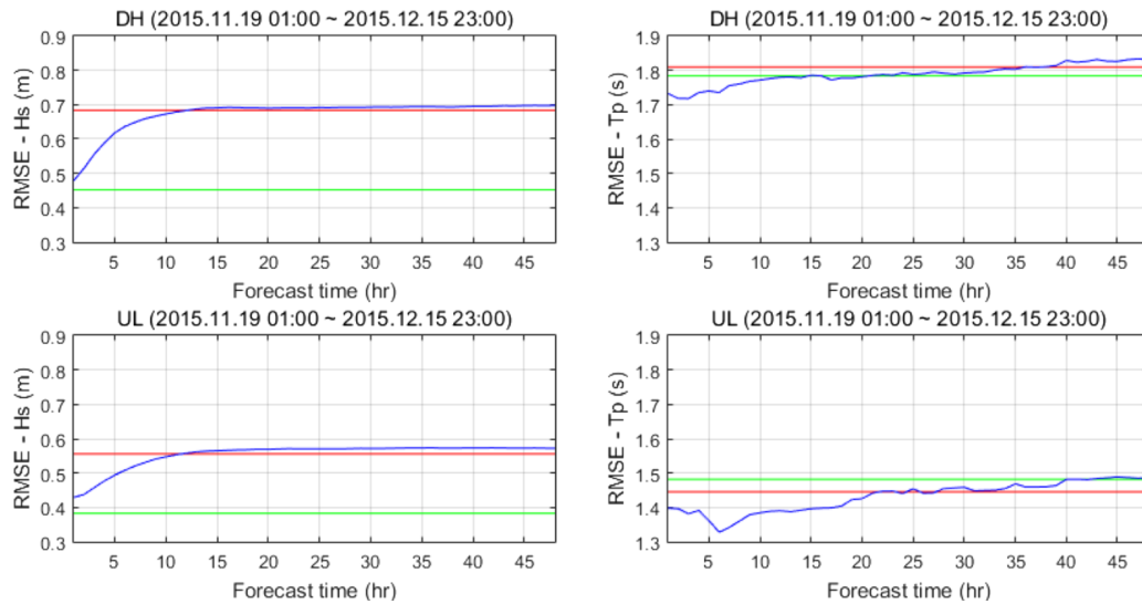
FIGURE 1.2: RMSE in significant wave height (left) and period (right) from two different observation locations. Figure 30 from Caires, Kim, and Groeneweg, 2018.
