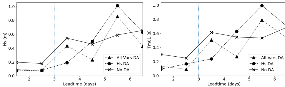
FIGURE 5.5: RMSE in H_s (left) and T_{m01} (right) analysis ensemble mean at the buoy location as a function of leadtime. RMSE is calculated over a 24hr period. Results shown for no DA (solid line), H_s DA (dashed line) and all vars DA (black dotted line). Blue dotted line indicates the end of the assimilation window.
