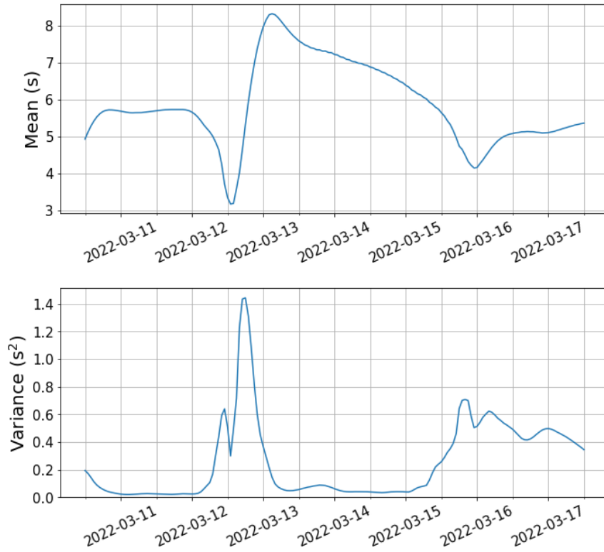
FIGURE 4.2: Timeseries of forecast (top) T_{m01} ensemble mean and (bottom) variance at the buoy location from the model run starting on the 10/03/2022.
