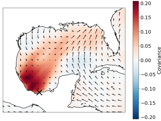
FIGURE 4.3: Colours showing spatial covariance of H_s at the buoy with H_s in the field at 12Z 12/03/2022. Arrows showing wind averaged over prior 24 hours.
