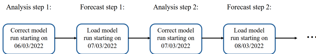
FIGURE 3.9: Schematic of the forecast and analysis steps from the ETKF scheme
