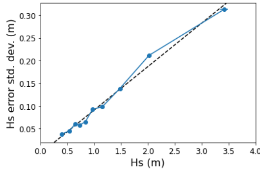
FIGURE 4.9: A plot of H_s error standard deviation against H_s . Calculated using observations from a period spanning 05/10/2021-13/04/2022
