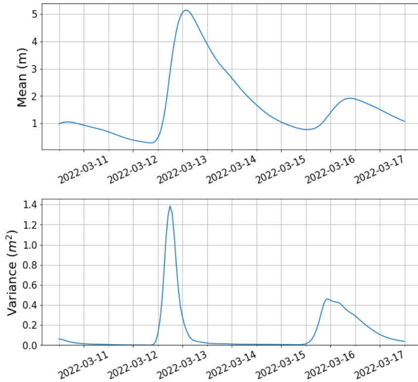
FIGURE 4.1: Timeseries of forecast (top) H_s ensemble mean and (bottom) variance at the buoy location from the model run starting on the 10/03/2022.
