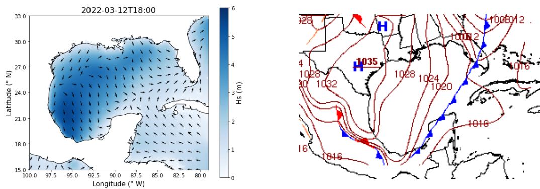
FIGURE 3.4: Left: H_s
