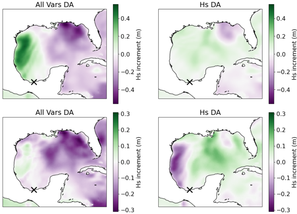
FIGURE 4.10: Hs increments at 12Z 15/03/2022 from all vars DA (left) and Hs DA (right). Taken from 12Z 10/03/2022 forecast run ensemble member 10 (top) and ensemble mean (bottom). The buoy location is marked with a cross.
