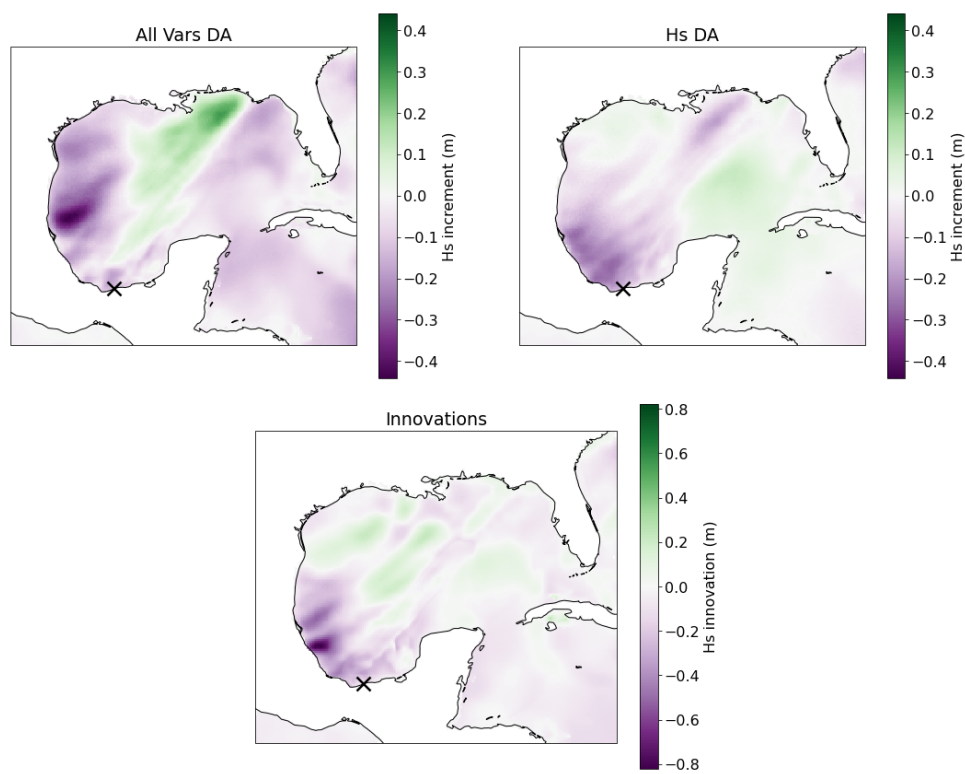
FIGURE 5.3: H_s ensemble mean increments at 12Z 12/03/2022 from all vars DA (top left) and H_s DA (top right), and H_s innovations from the same time (bottom). Taken from 12Z 10/03/2022 forecast run. The buoy location is marked with a cross.
