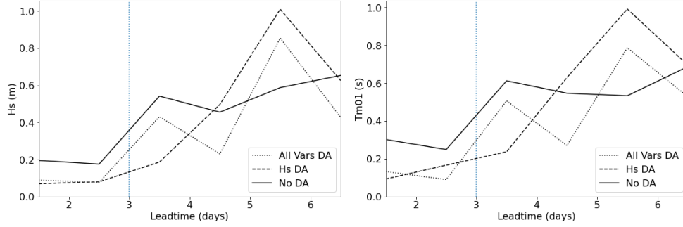
FIGURE 5.5: RMSE in H_s (left) and T_{m01} (right) ensemble mean at the buoy location as a function of leadtime. RMSE is calculated over a 24hr period. Results shown for no DA (solid line), H_s DA (dashed line) and all vars DA (black dotted line). Blue dotted line indicates the end of the assimilation window.
