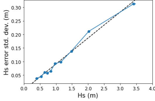
FIGURE 4.8: A plot of H_s error standard deviation against H_s .
