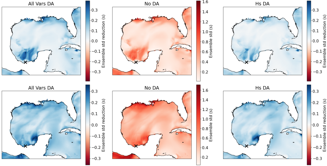
FIGURE 5.10: Ensemble standard deviation in T_{m01} at 12Z 11/03/2022, taken from 12Z 06/03/2022 (top) and 12Z 10/03/2022 (bottom) model runs. Middle panel shows standard deviation from no DA, side panels show standard deviation reduction from all vars DA (left) and H_s DA (right).
