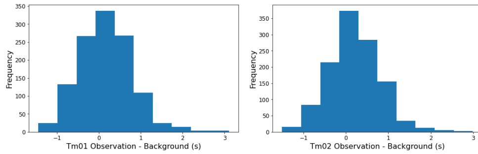
FIGURE 4.10: Observation minus background histograms for T_{m01} (left) and T_{m02} (right).
