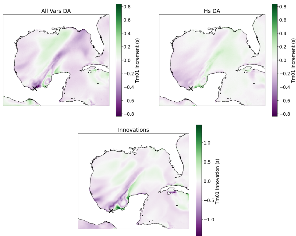
FIGURE 5.4: T_{m01} ensemble mean increments at 12Z 12/03/2022 from all vars DA (top left) and H_s DA (top right), and T_{m01} innovations from the same time (bottom). Taken from 12Z 10/03/2022 forecast run. The buoy location is marked with a cross.
