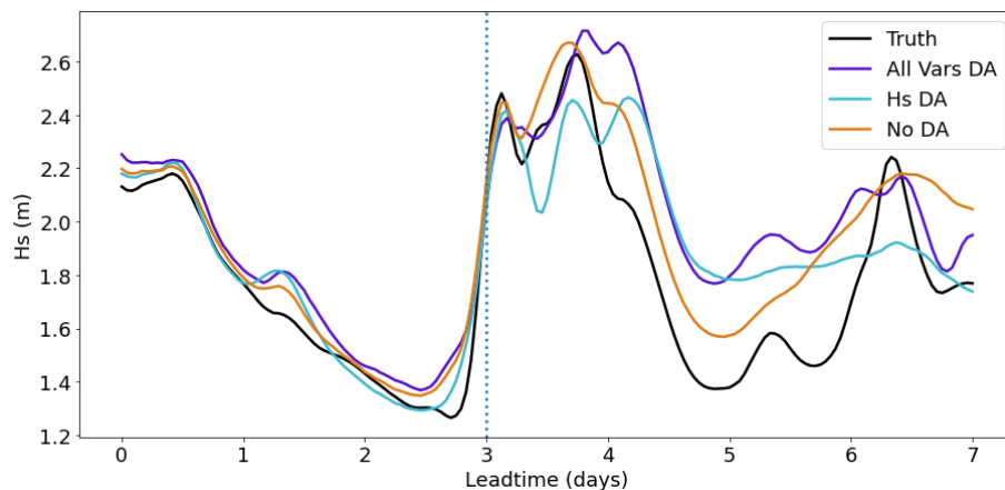
FIGURE 5.2: Timeseries of significant wave height at 30^{\circ}\text{N } 80^{\circ}\text{ W} from 12Z 09/03/2022 model run. Truth is shown in black, and all vars DA, H_s DA and no DA ensemble means are shown in dark blue, light blue and orange respectively. Blue dotted line indicates the end of the assimilation window.
