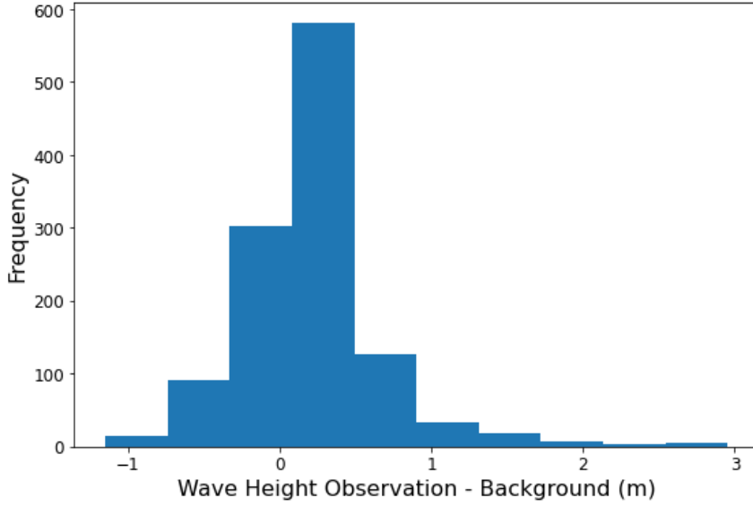
FIGURE 4.7: Observation - background histogram for significant wave height, from the forecast window 06/03/2022 to 19/03/2022.
