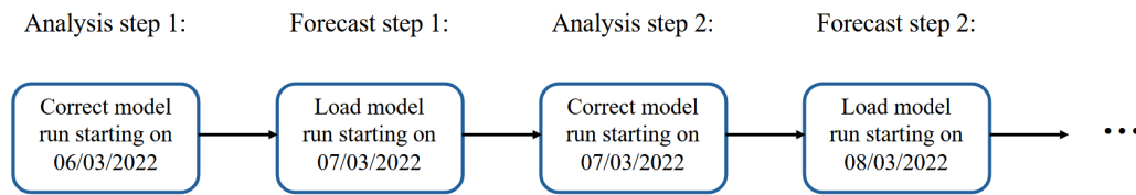
FIGURE 3.9: Schematic of the forecast and analysis steps from the data assimilation method used in this study.
