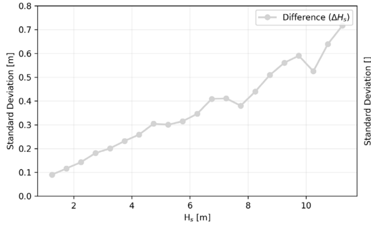
FIGURE 4.8: Observation difference standard deviation in significant wave height as a function of significant wave height. Figure 2 from Houghton et al. (2023)
