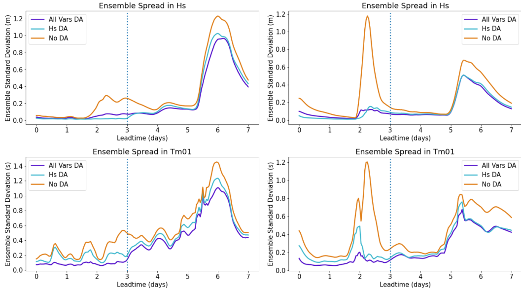
FIGURE 5.8: Timeseries of ensemble standard deviation in significant wave height (top) and T_{m01} (bottom) at the buoy location for 12Z 06/03/2022 (left) and 12Z 10/03/2022 (right) model runs.
