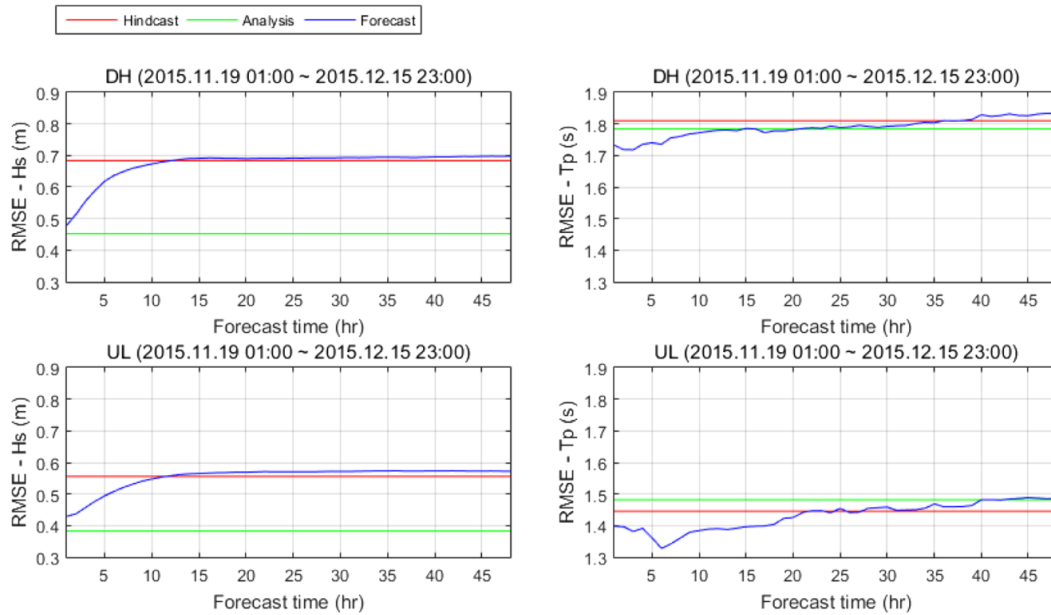
FIGURE 1.2: RMSE in wave height (left) and period (right) from two different observation locations. Figure 30 from Caires et al. (2018) .
