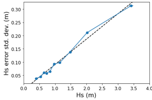
FIGURE 4.9: A plot of significant wave height error standard deviation against significant wave height. Calculated using observations from a period spanning 05/10/2021-13/04/2022
