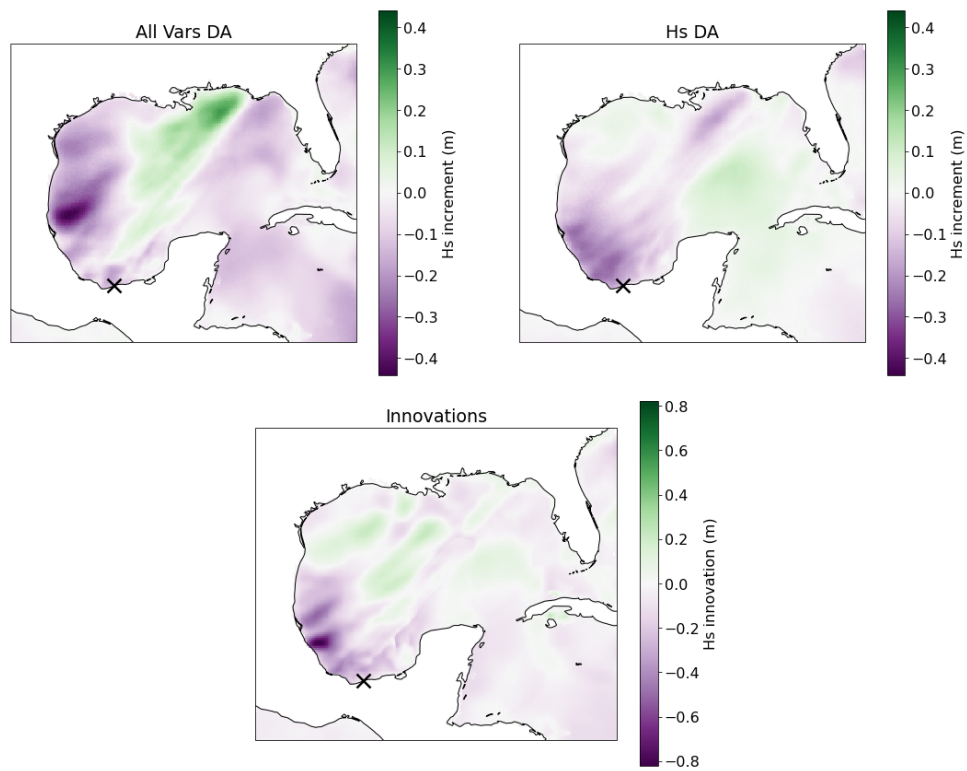
FIGURE 5.3: Significant wave height ensemble mean increments at 12Z 12/03/2022 from all vars DA (top left) and H_s DA (top right), and significant wave height innovations from the same time (bottom). Taken from 12Z 10/03/2022 forecast run. The buoy location is marked with a cross.
