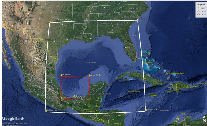
FIGURE 3.1: Model domains shown on map.
