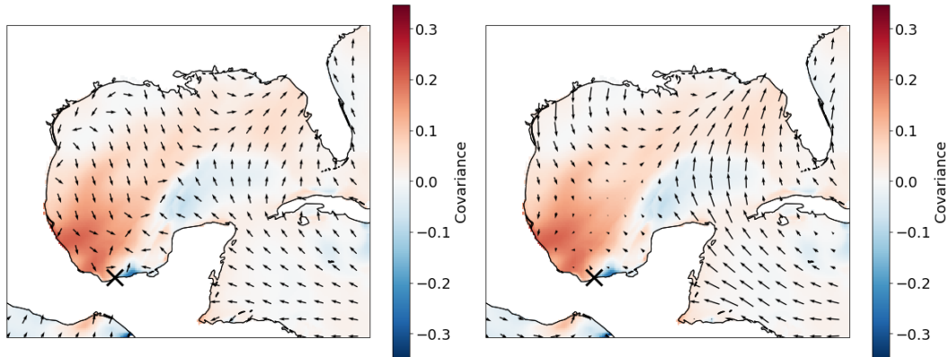
FIGURE 4.6: Cross-covariance between significant wave height at the buoy and T_{m01} in the field at 12Z 12/03/2022. Arrows show wave direction (left) and wind (right).
