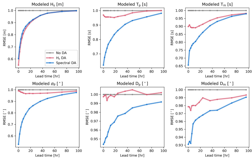
FIGURE 1.3: RMSE from spectral DA and significant wave height ( H_s ) DA, normalised by the RMSE without DA. Results shown for significant wave height H_s , peak period T_p , mean period T_m , directional spread \sigma_\theta , peak direction D_p and mean direction D_m . Figure 3 from Houghton et al. (2022) .
