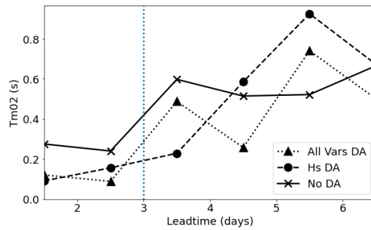
FIGURE A.2: RMSE in T_{m02} ensemble mean at the buoy location as a function of leadtime. RMSE is calculated over a 24hr period. Results shown for no DA (solid line), H_s DA (dashed line) and all vars DA (black dotted line). Blue dotted line indicates the end of the assimilation window. Equivalent to figure 5.5.
