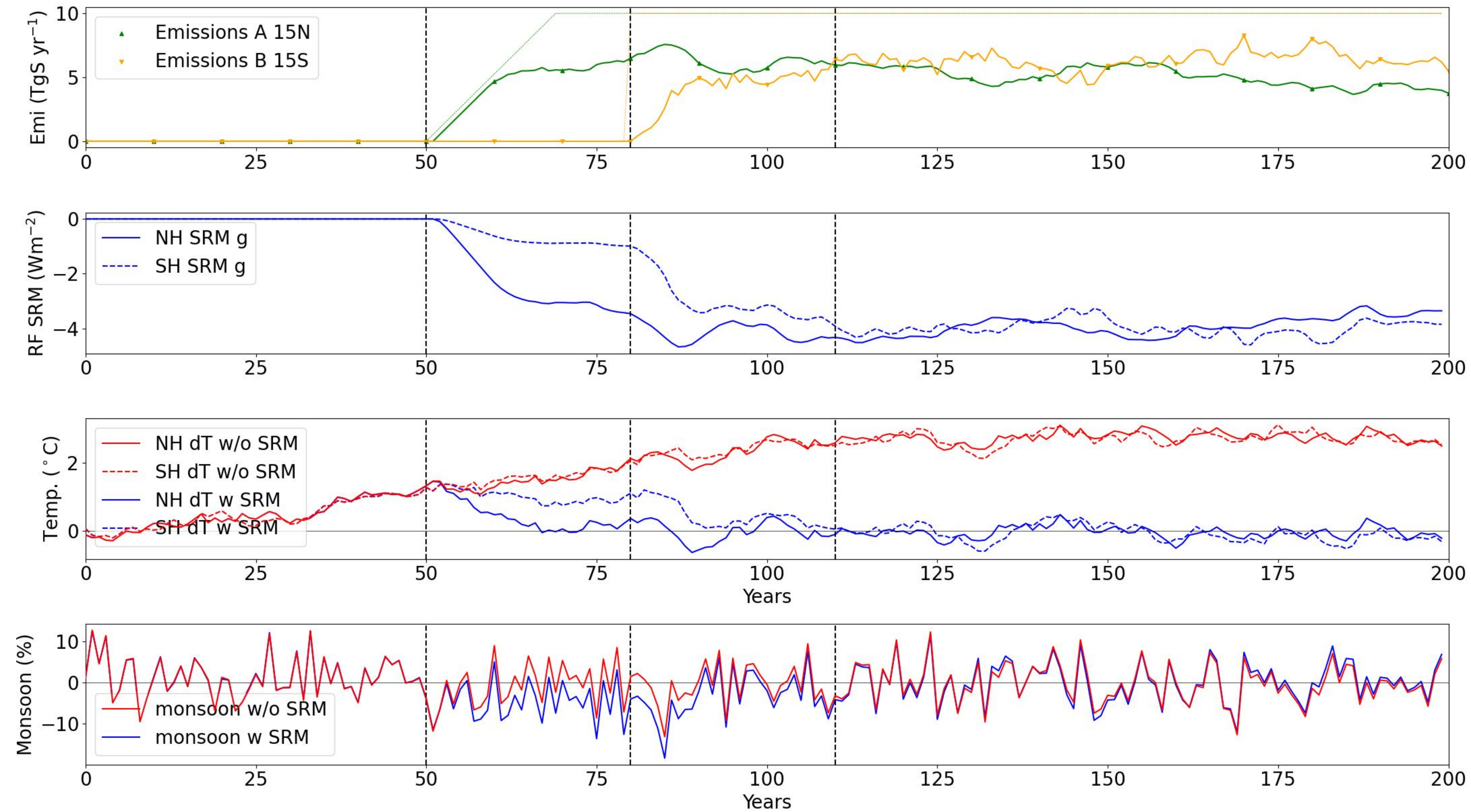
Controlling global SAI - A NHST 0.0 - B monsoon 0.0 ### EXP: 4c cki= 0.5
