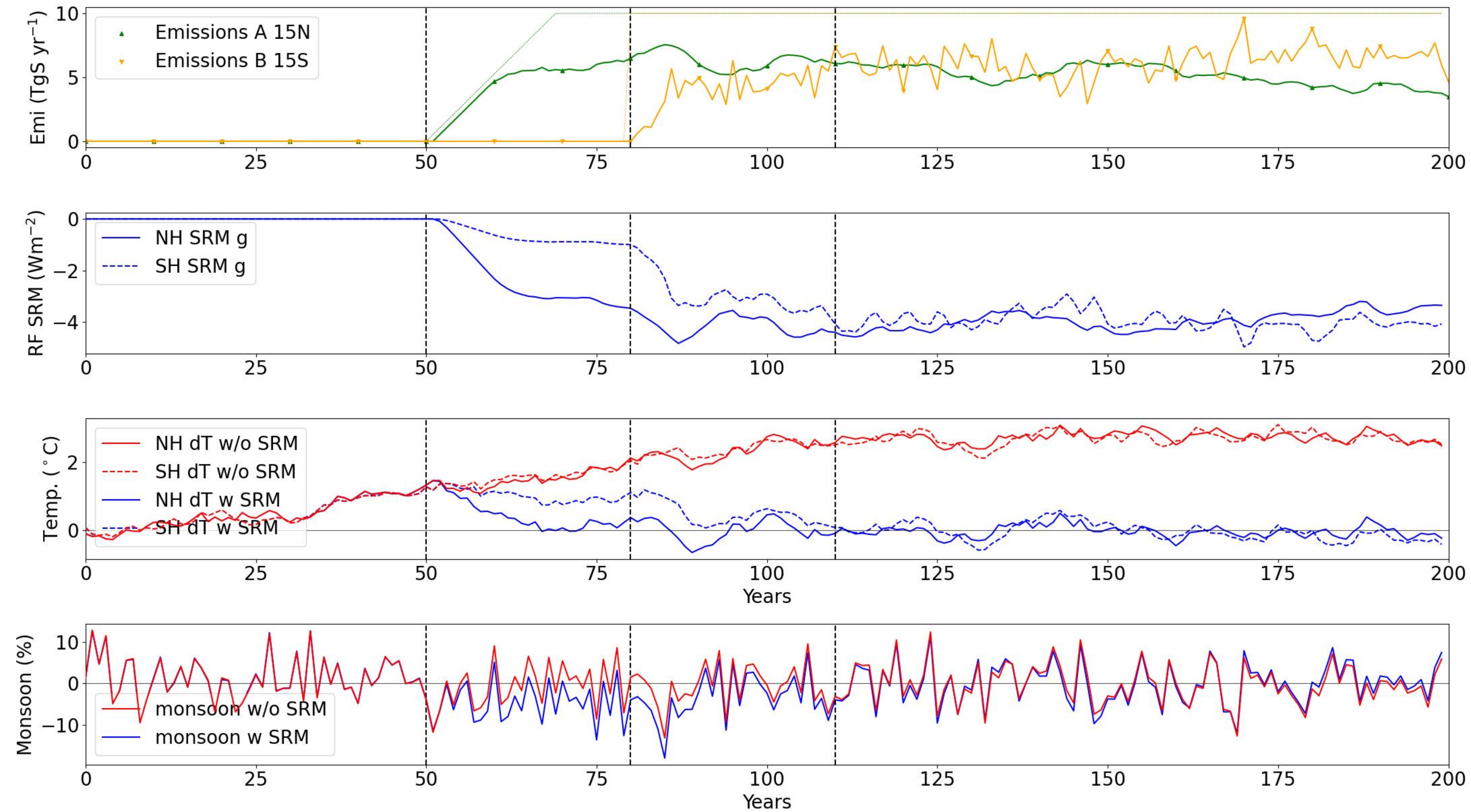
Controlling global SAI - A NHST 0.0 - B monsoon 0.0 ### EXP: 4c cki= 2.0
