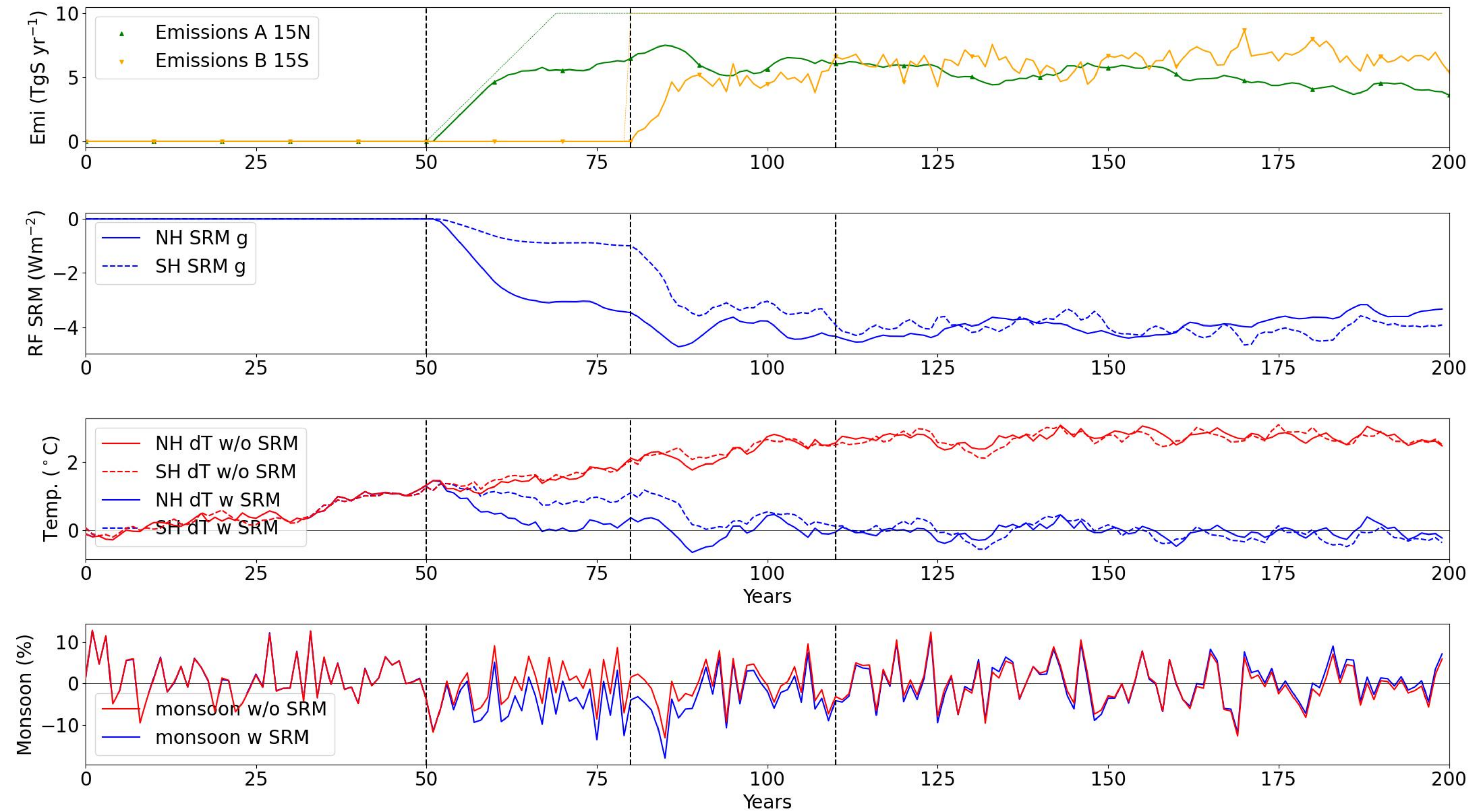
Controlling global SAI - A NHST 0.0 - B monsoon 0.0 ### EXP: 4c REFERENCE
