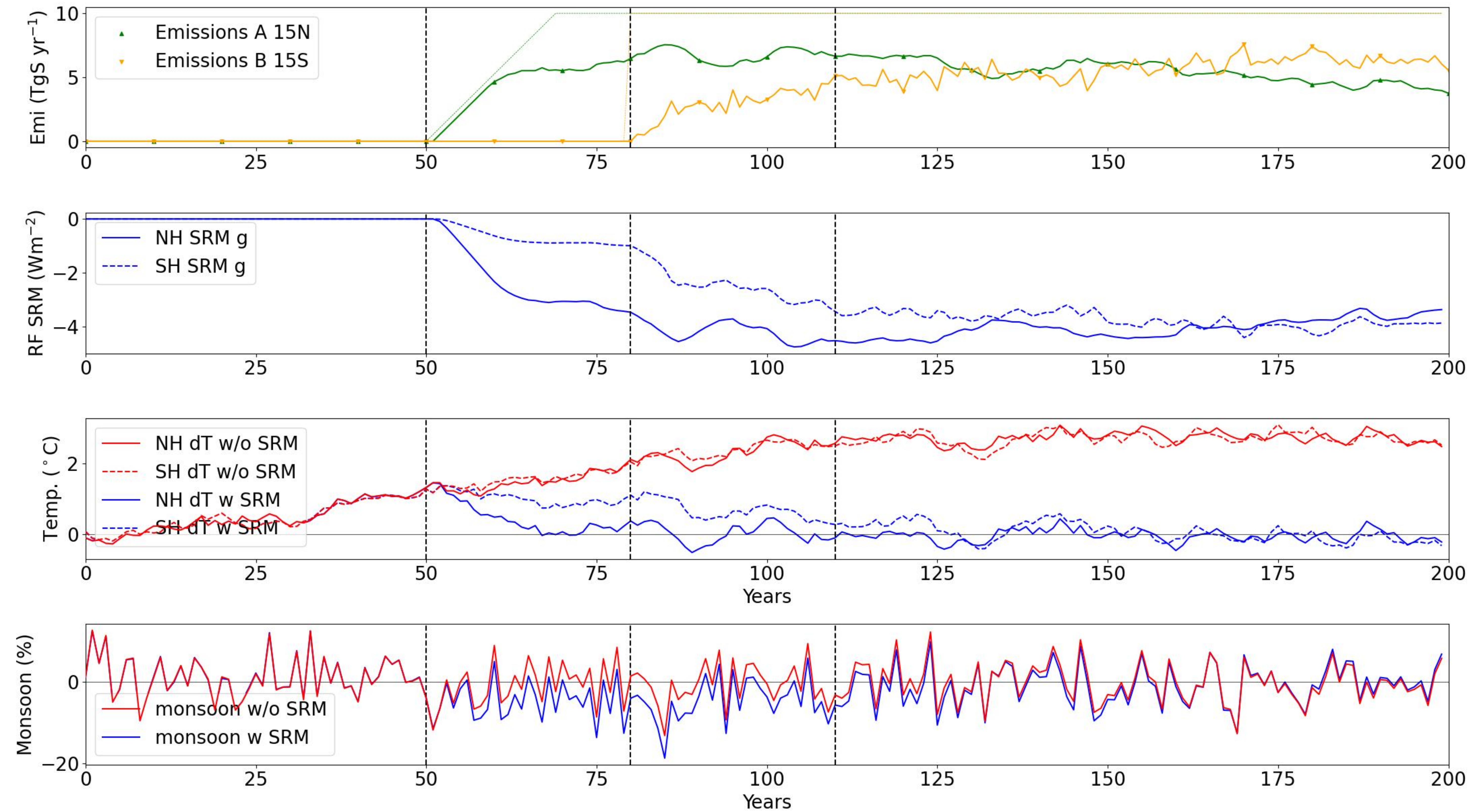
Controlling global SAI - A NHST 0.0 - B monsoon 0.0 ### EXP: 4c ckp= 0.5
