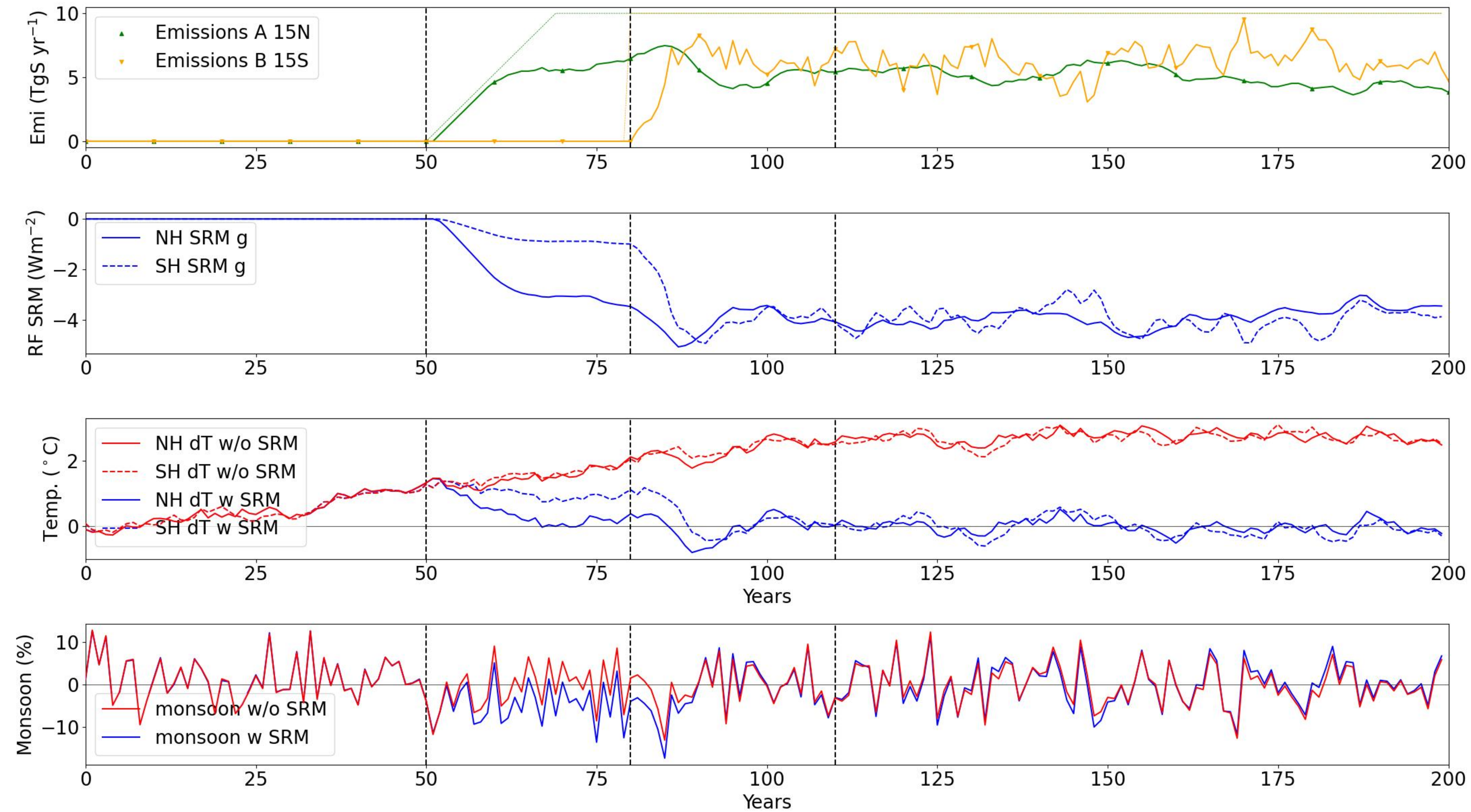
Controlling global SAI - A NHST 0.0 - B monsoon 0.0 ### EXP: 4c ckp= 2.0
