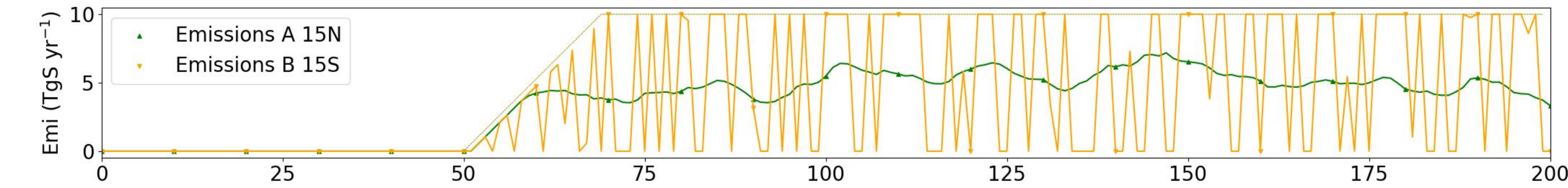
Controlling global SAI - A NHST 0.0 - B monsoon 0.0 ### EXP: 24c
