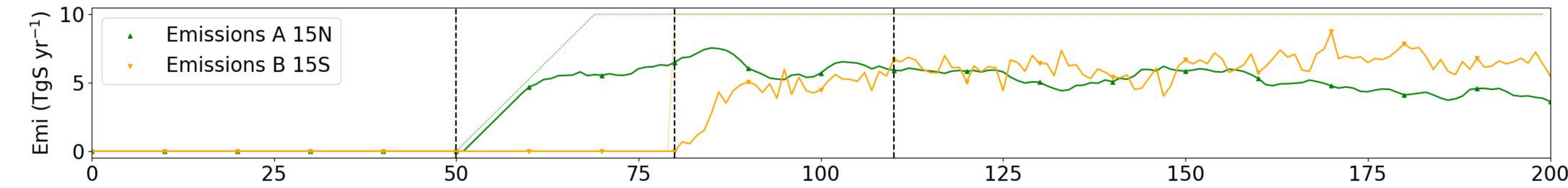
Controlling global SAI - A NHST 0.0 - B monsoon 0.0 ### EXP: 4c
