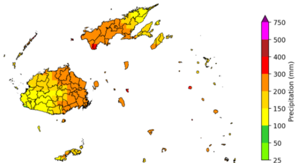
Cyclone Yasa: 2-day rainfall Average over whole country: 199 mm
