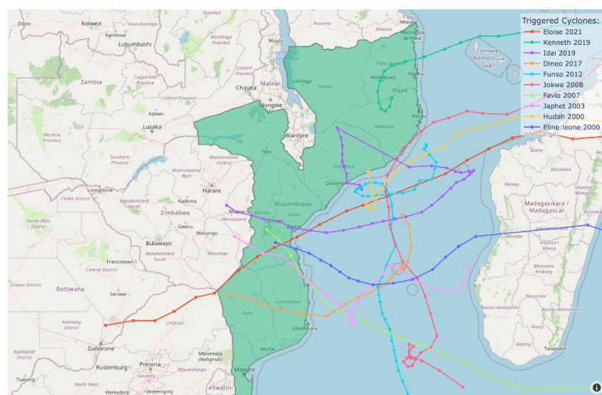
Figure 2. Historical tracks of cyclones in Mozambique 2000-2022
