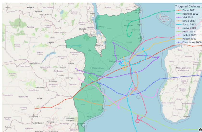
Figure 2. Historical tracks of cyclones in Mozambique since 2000
