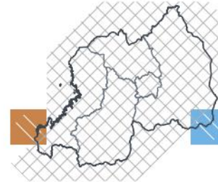
SON 2026 — lead 1 mo 1-in-3 wet · 67th pct
