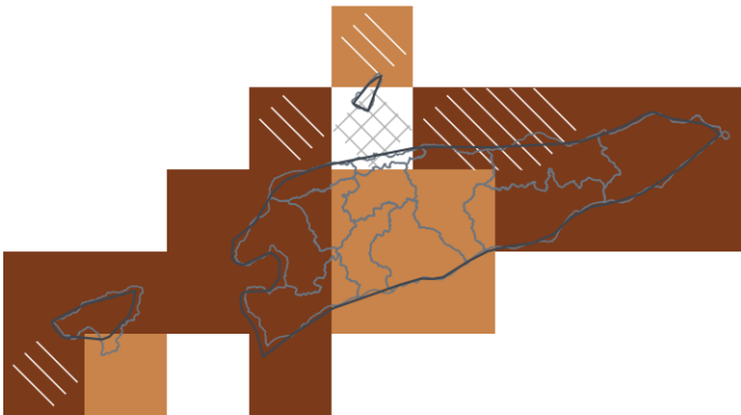
DJF 2026/27 — lead 4 mo — 9th pct
