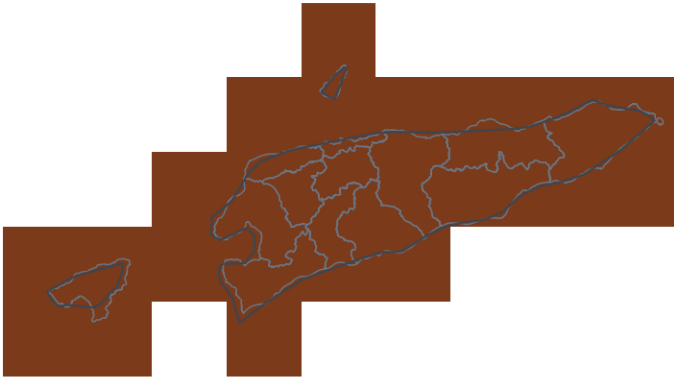
OND 2026 — lead 2 mo — 0th pct ← driest overall
