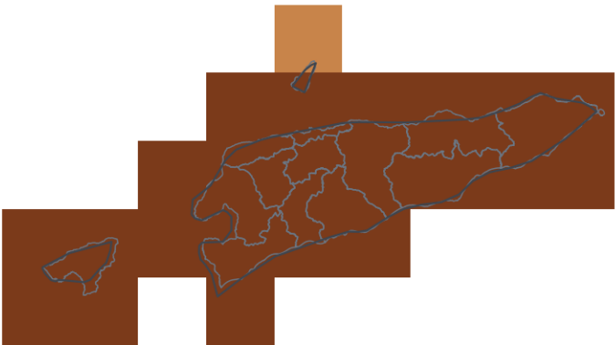
NDJ 2026/27 — lead 3 mo — 3rd pct
