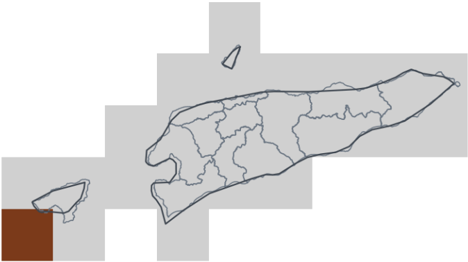
SON 2026 — lead 1 mo — 0th pct
