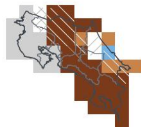
NDJ 2026/27 — lead 3 mo 1-in-15 dry · 4th pct
