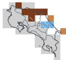
DJF 2026/27 — lead 4 mo off-season
