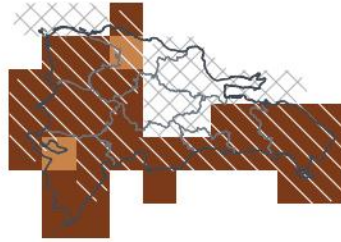
ASO 2026 — in season 1-in-23 dry · 2nd pct
