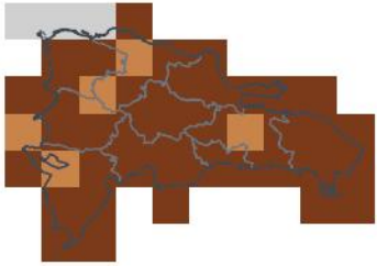
JJA 2026 — in season 1-in-15 dry · 4th pct
