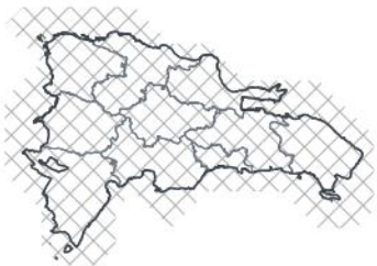
OND 2026 — lead 2 mo 1-in-9 dry · 9th pct
