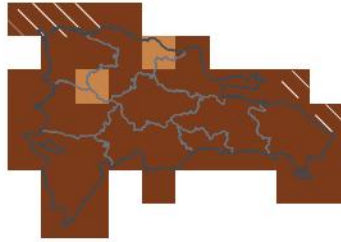
JAS 2026 — in season 1-in-15 dry · 4th pct
