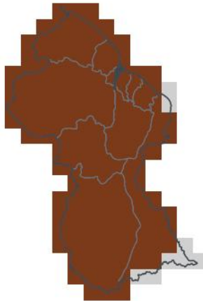
ASO 2026 — in season 1-in-23 dry · 2nd pct
