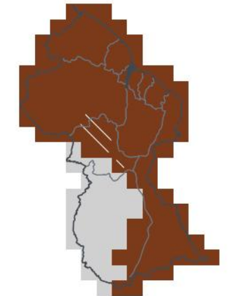
NDJ 2026/27 — lead 3 mo 1-in-46 dry · 0th pct
