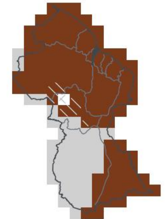
DJF 2026/27 — lead 4 mo 1-in-46 dry · 0th pct
