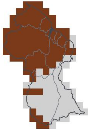
SON 2026 — lead 1 mo 1-in-46 dry · 0th pct
