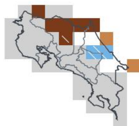
DJF 2026/27 — lead 4 mo off-season
