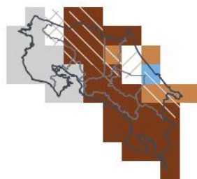
NDJ 2026/27 — lead 3 mo 1-in-15 dry · 4th pct
