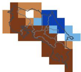
JJA 2026 — in season 1-in-15 dry · 4th pct
