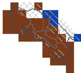
ASO 2026 — in season 1-in-23 dry · 2nd pct
