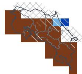
SON 2026 — lead 1 mo 1-in-23 dry · 2nd pct
