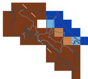
JAS 2026 — in season 1-in-23 dry · 2nd pct
