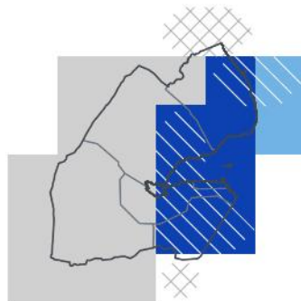
NDJ 2026/27 — lead 3 mo 1-in-12 wet · 93rd pct
