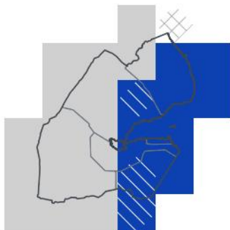
OND 2026 — lead 2 mo 1-in-15 wet · 96th pct
