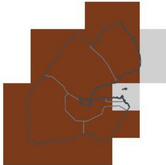
JJA 2026 — in season 1-in-46 dry · 0th pct
