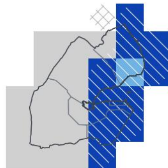
DJF 2026/27 — lead 4 mo 1-in-15 wet · 96th pct
