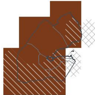
ASO 2026 — in season 1-in-46 dry · 0th pct
