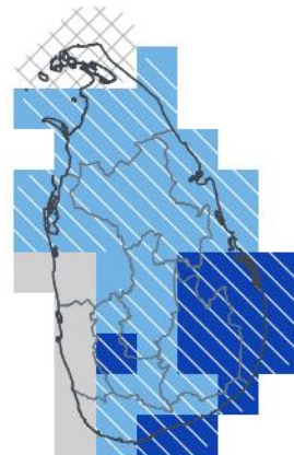
DJF 2026/27 — lead 4 mo 1-in-7 wet · 87th pct
