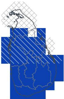
OND 2026 — lead 2 mo 1-in-46 wet · 100th pct
