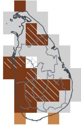
JAS 2026 — in season 1-in-46 dry · 0th pct
