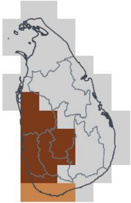
JJA 2026 — in season 1-in-46 dry · 0th pct
