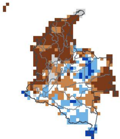
JJA 2026 — in season 1-in-15 dry · 4th pct
