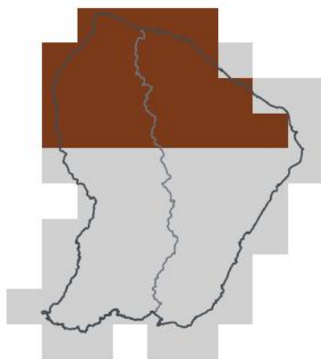
JAS 2026 — in season off-season
