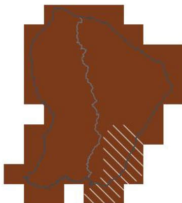
DJF 2026/27 — lead 4 mo 1-in-46 dry · 0th pct
