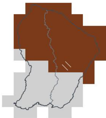
OND 2026 — lead 2 mo 1-in-46 dry · 0th pct
