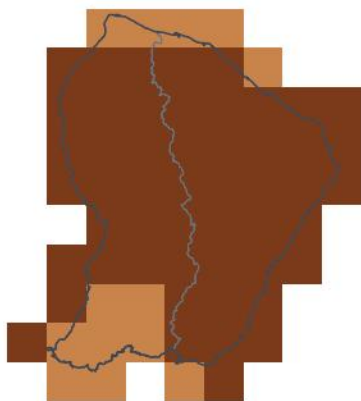
JJA 2026 — in season 1-in-15 dry · 4th pct
