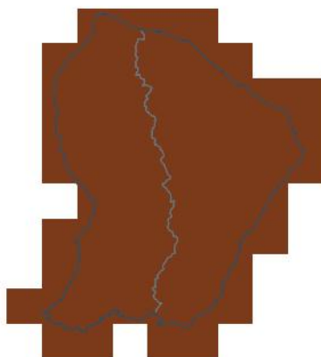
NDJ 2026/27 — lead 3 mo 1-in-46 dry · 0th pct
