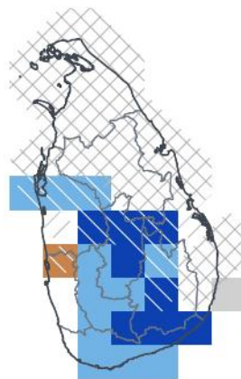
ASO 2026 — in season 1-in-4 wet · 73rd pct
