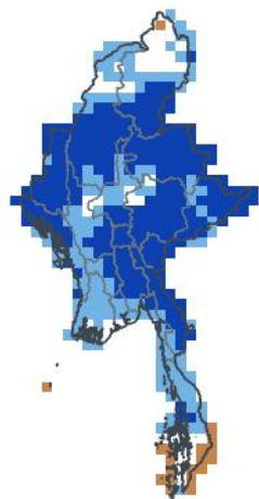
JJA 2026 — in season 1-in-46 wet · 100th pct
