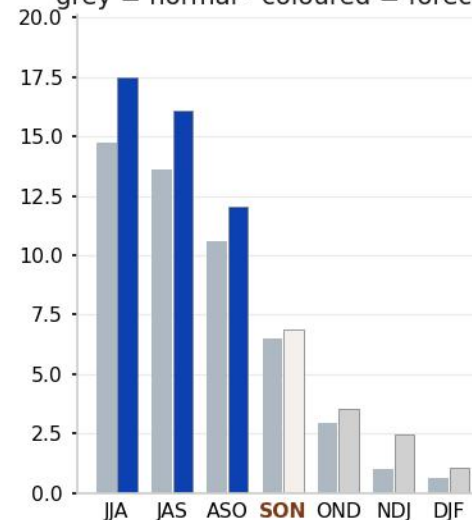
Country-mean rainfall (mm/day) grey = normal · coloured = forecast
