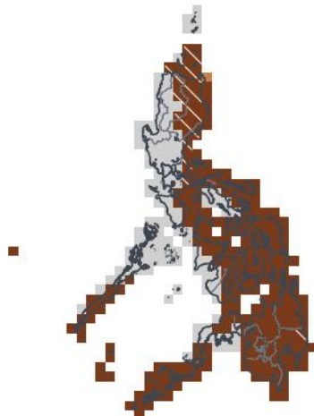
DJF 2026/27 — lead 4 mo 1-in-46 dry · 0th pct
