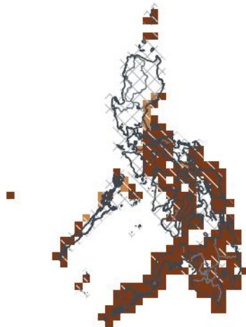
ASO 2026 — in season 1-in-23 dry · 2nd pct
