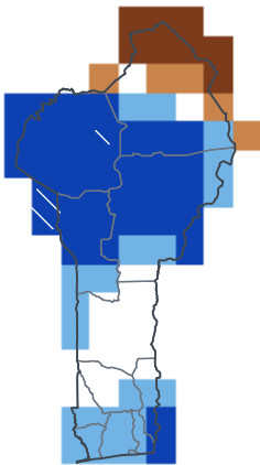
JJA 2026 — in season 1-in-9 wet · 91st pct
