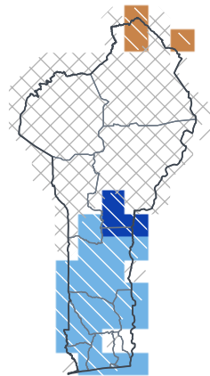
SON 2026 — lead 1 mo 1-in-9 wet · 91st pct
