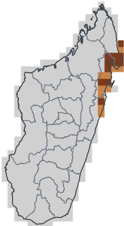
JAS 2026 — in season off-season
