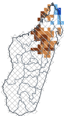
DJF 2026/27 — lead 4 mo 1-in-23 dry · 2nd pct
