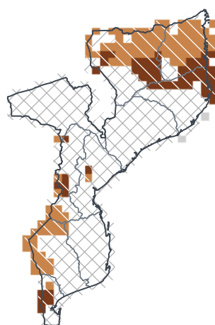
OND 2026 — lead 2 mo 1-in-46 dry · 0th pct
