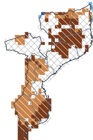
DJF 2026/27 — lead 4 mo 1-in-23 dry · 2nd pct
