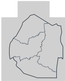
JAS 2026 — in season off-season
