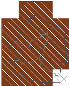
NDJ 2026/27 — lead 3 mo 1-in-46 dry · 0th pct
