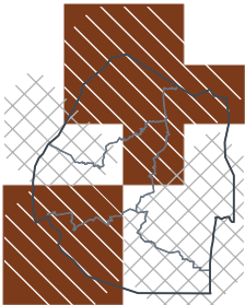
OND 2026 — lead 2 mo 1-in-15 dry · 4th pct
