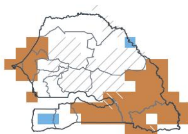
JAS 2026 — in season 1-in-3 dry · 38th pct
