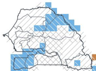
ASO 2026 — in season 1-in-3 wet · 62nd pct
