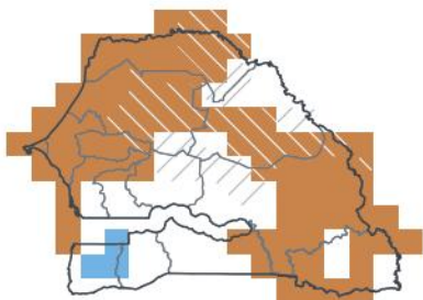
JJA 2026 — in season 1-in-3 dry · 33rd pct
