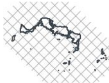
SON 2026 — lead 1 mo 1-in-4 dry · 22nd pct
