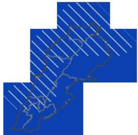
OND 2026 — lead 2 mo 1-in-46 wet · 100th pct
