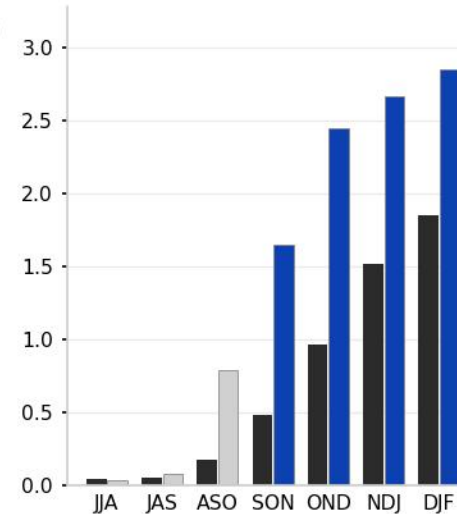
Country-mean rainfall (mm/day) black = normal · coloured = forecast
