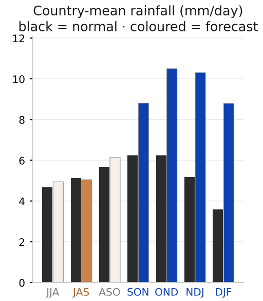
DJF 2026/27 — lead 4 mo 1-in-23 wet · 98th pct
