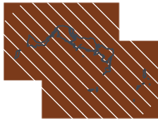
ASO 2026 — in season 1-in-23 dry · 2nd pct
