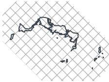
DJF 2026/27 — lead 4 mo 1-in-46 wet · 100th pct
