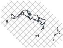
NDJ 2026/27 — lead 3 mo 1-in-46 wet · 100th pct
