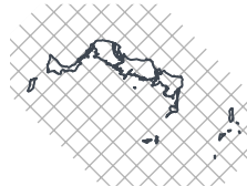
SON 2026 — lead 1 mo 1-in-4 dry · 22nd pct
