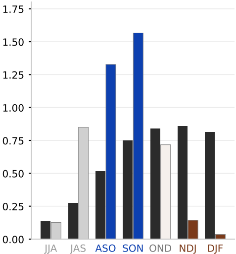
Country-mean rainfall (mm/day) black = normal · coloured = forecast
