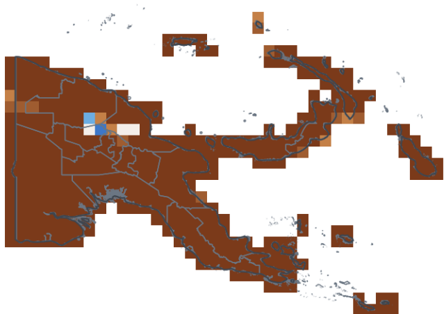
SON 2026 — lead 1 mo — mean 6th pct ← driest overall
