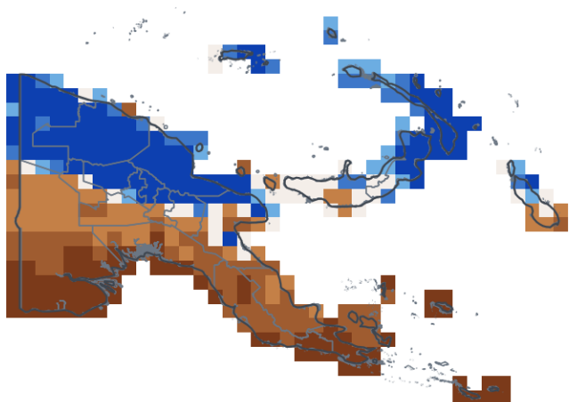
NDJ 2026/27 — lead 3 mo — mean 48th pct
