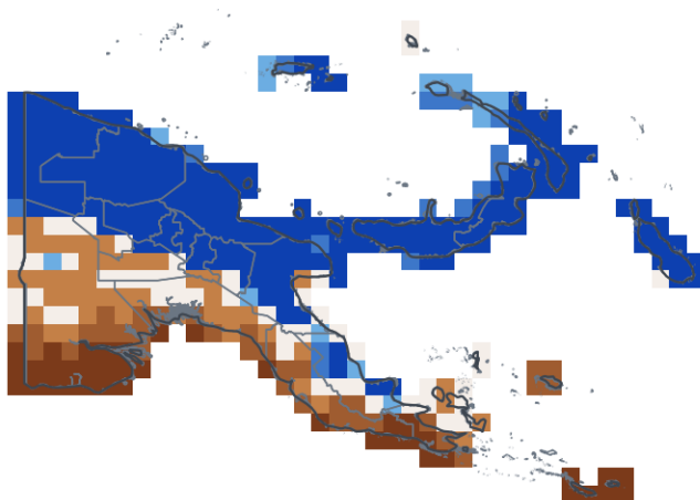
DJF 2026/27 — lead 4 mo — mean 64th pct
