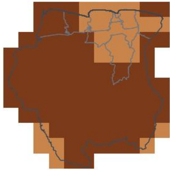
JJA 2026 — in season 1-in-12 dry · 7th pct
