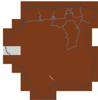
DJF 2026/27 — lead 4 mo 1-in-46 dry · 0th pct
