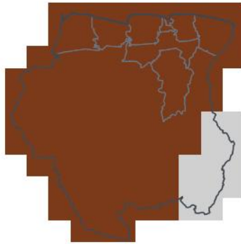
JAS 2026 — in season 1-in-46 dry · 0th pct
