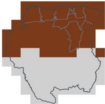
OND 2026 — lead 2 mo 1-in-46 dry · 0th pct
