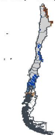
OND 2026 — lead 2 mo 1-in-2 dry · 49th pct
