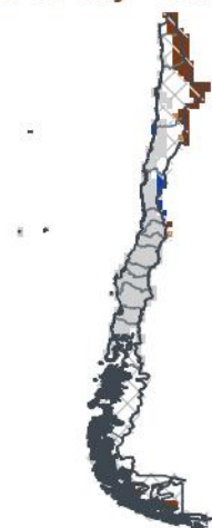
DJF 2026/27 — lead 4 mo 1-in-46 dry · 0th pct
