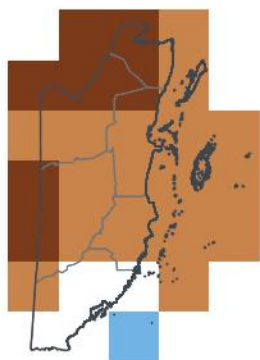
JJA 2026 — in season 1-in-5 dry · 18th pct
