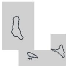
SON 2026 — lead 1 mo off-season
