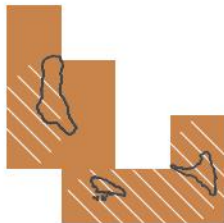
NDJ 2026/27 — lead 3 mo 1-in-5 dry · 20th pct
