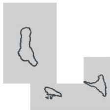
JAS 2026 — in season off-season
