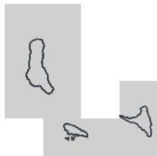
ASO 2026 — in season off-season
