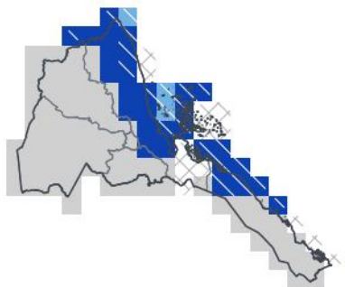
OND 2026 — lead 2 mo off-season
