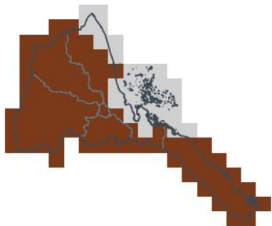
JJA 2026 — in season 1-in-46 dry · 0th pct
