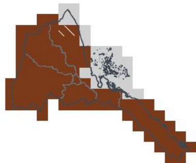
JAS 2026 — in season 1-in-46 dry · 0th pct
