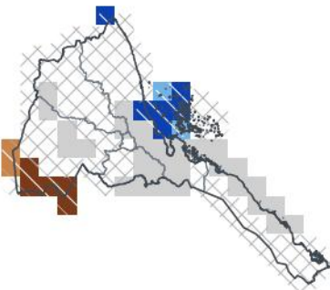
SON 2026 — lead 1 mo 1-in-3 dry · 36th pct
