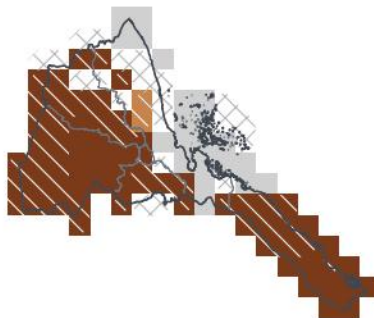
ASO 2026 — in season 1-in-46 dry · 0th pct
