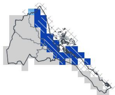
NDJ 2026/27 — lead 3 mo off-season
