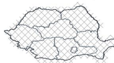
SON 2026 — lead 1 mo 1-in-46 wet · 100th pct
