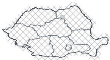
OND 2026 — lead 2 mo 1-in-23 wet · 98th pct
