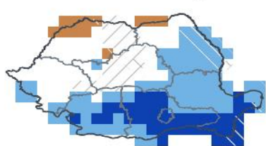
JAS 2026 — in season 1-in-4 wet · 78th pct
