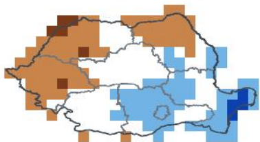
JJA 2026 — in season 1-in-2 dry · 47th pct
