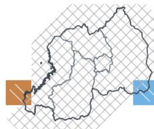
SON 2026 — lead 1 mo 1-in-3 wet · 67th pct
