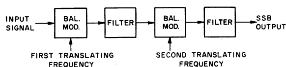
Fig. 1—Filter method of SSB generation.
