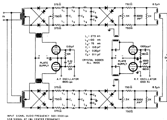
Fig. 7—Single-sideband generator.
