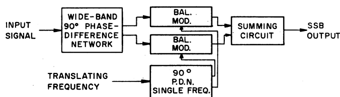
Fig. 2—Phasing method of SSB generation.
