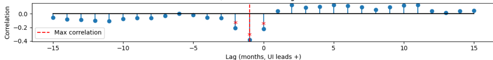
Cross-correlation of Residuals (Max r = -0.38 at lag -1)
