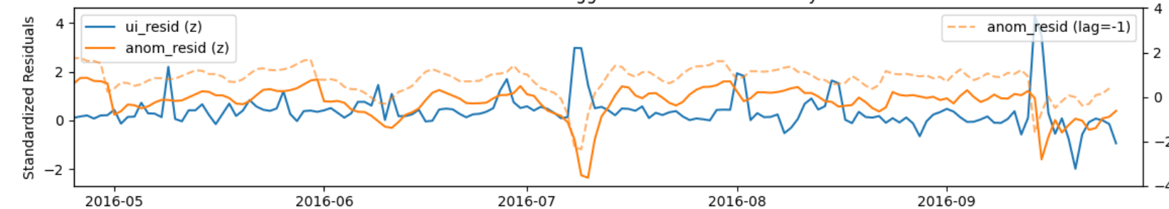
Cross-correlation of Residuals (Max r = -0.38 at lag -1)
