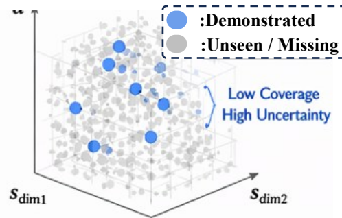
State-Action Space
