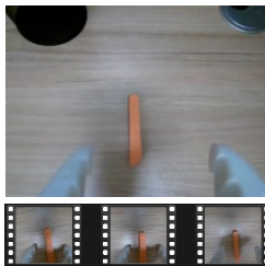
State-Action Space
