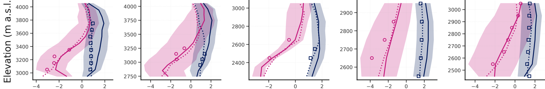
Gries (1962-2024) Clariden (1951-2024) Gietro (1967-2024) Schwarzberg (1956-2024) Forno (1955-1960)
