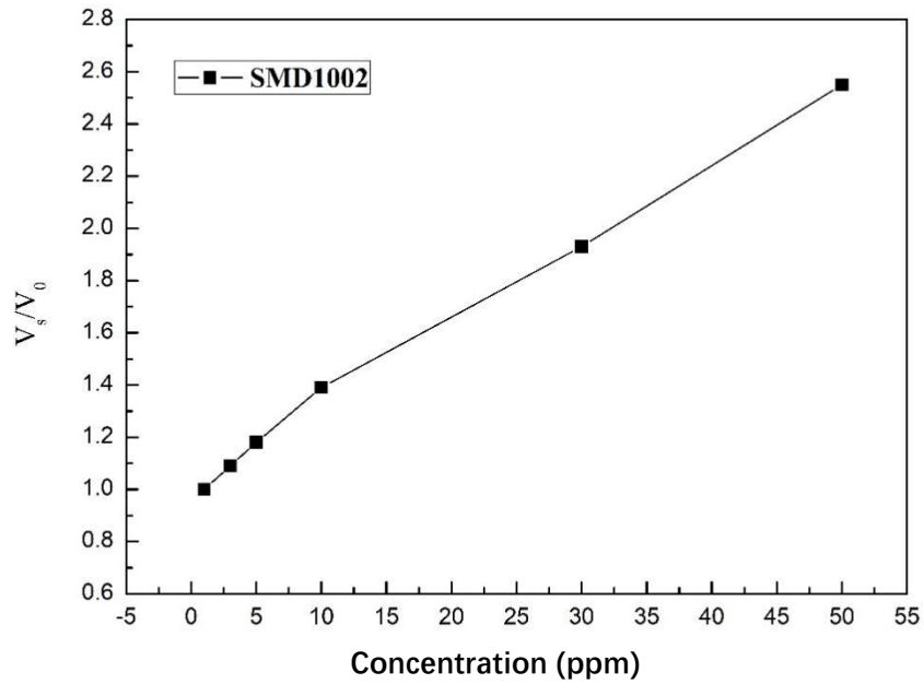
Figure 1 ammonia sensor sensitivity characteristic curve
