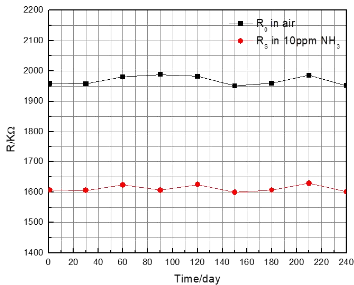
Figure 4 Long-term stability curve of the sensor
